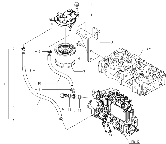
Fig.13. FUEL FILTER
