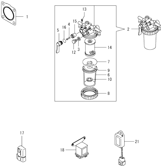
Fig.16. ACCESSORY
